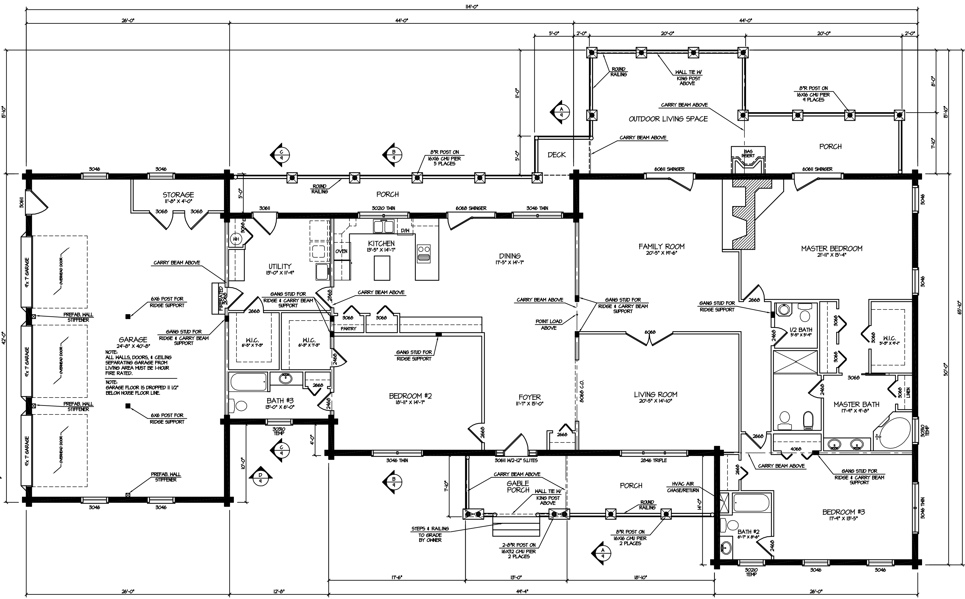
1st FLOOR PLAN 1/4" = 1'-0"
