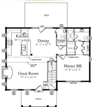
1st FLOOR PLAN (1,024 S.F.)
