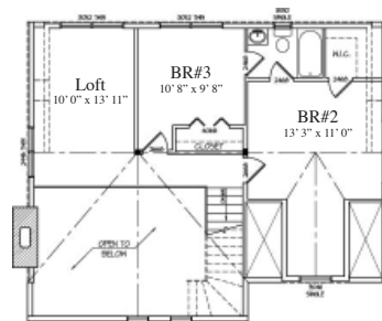
2nd FLOOR PLAN (640 S.F.)
